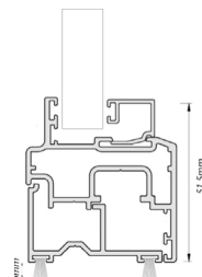
Door Threshold Detail
