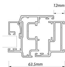
Door Outer Frame and Sash Detail
