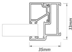
Door Outer Frame and Sash Detail
